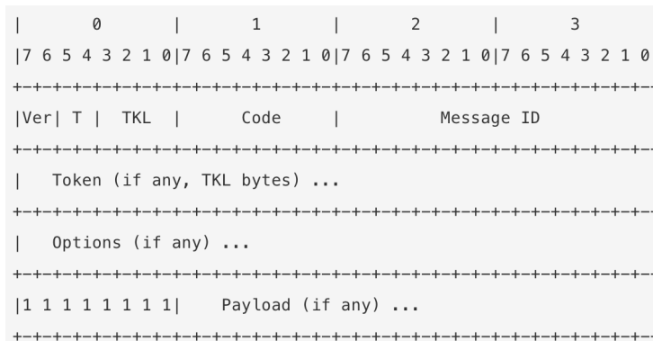
Figure 2-19. CoAP message format [64]
