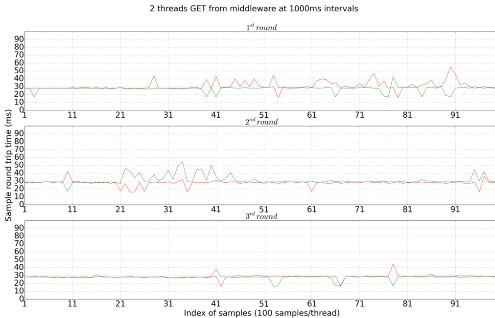
Figure 5-3. Two threads sending 100 GET requests (1000 milliseconds delay)
