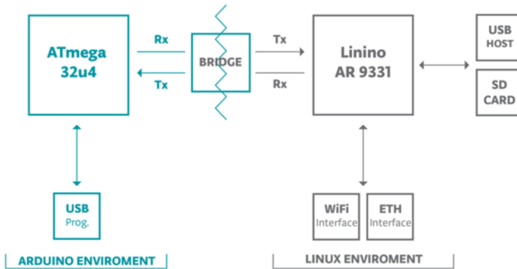
Figure 2-6. Arduino Yun Bridge [27]
