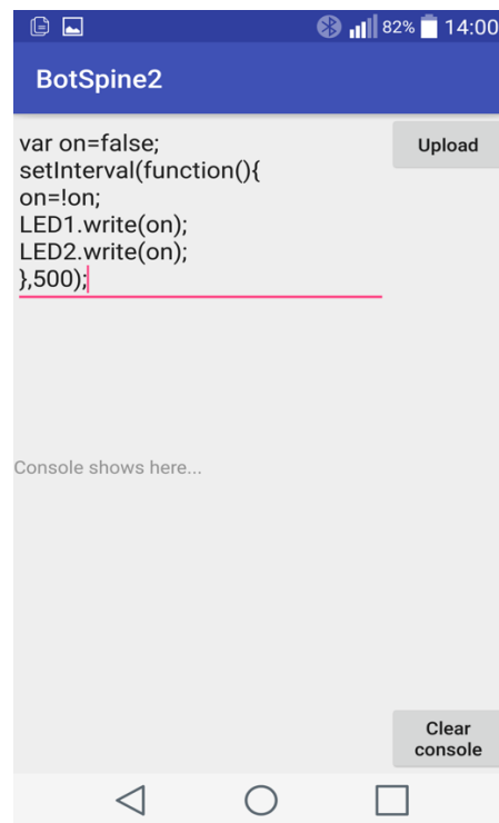
Figure 4-9. Example of BLE write in JavaScript
