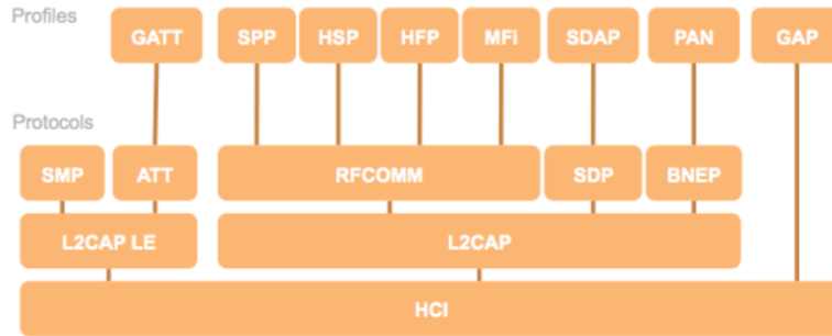
Figure 2-23. Bluetooth profiles and middle-layer protocols [14]
