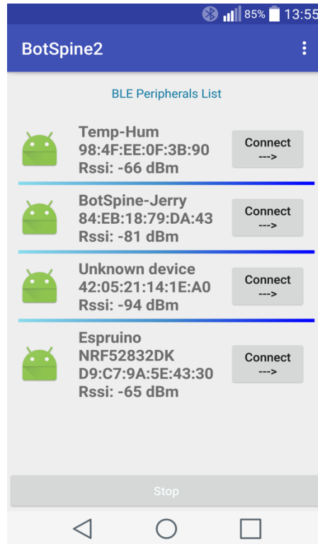
Figure 4-8. Example of BLE scanning in a mobile app
