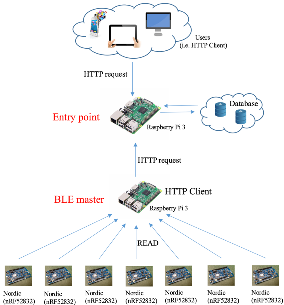
Figure 3-4. Sensing flow
