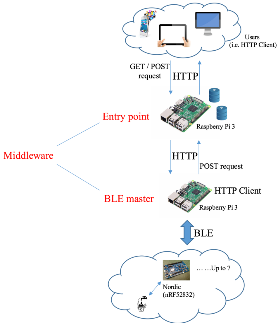
Figure 3-3. Simplified architecture
