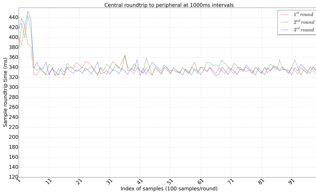
Figure 5-18. 100 sequential round trip to an endpoint (1 second delay)
