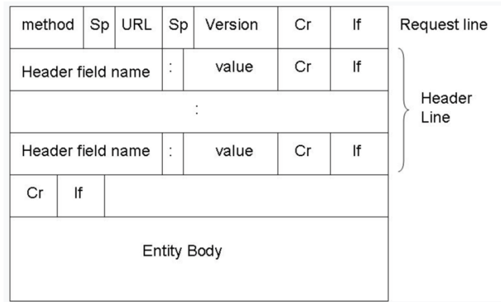
Figure 2-20. HTTP message format [1]
