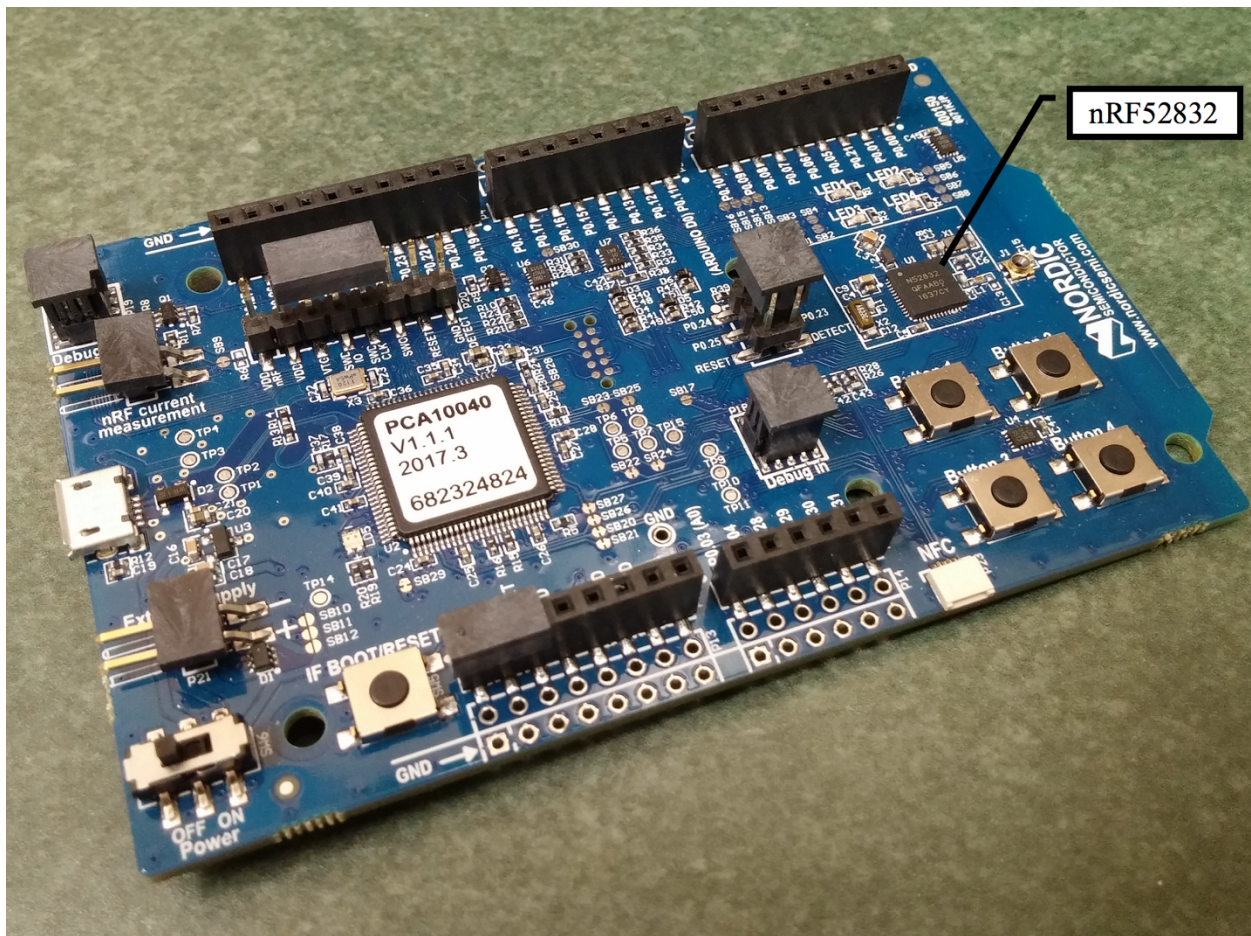
Figure 2-14. Nordic nRF52832 development board
