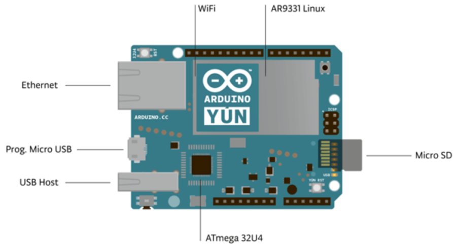
Figure 2-3. Arduino Yun layout [4]
