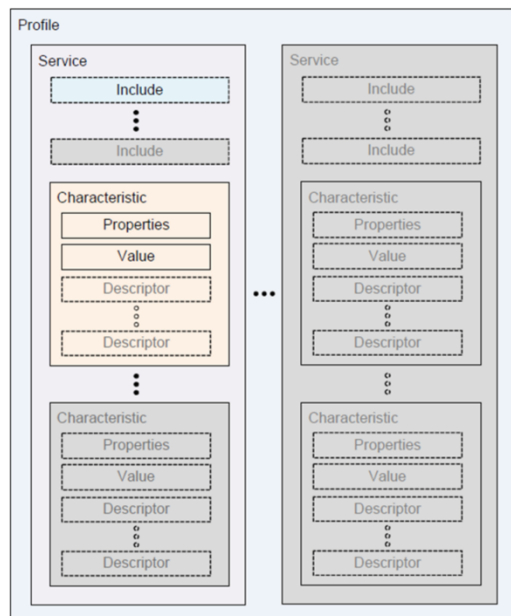
Figure 2-24. GATT profile hierarchy [12]
