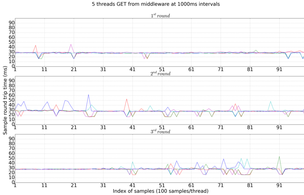
Figure 5-4. Five threads sending 100 GET requests (1000 milliseconds delay)
