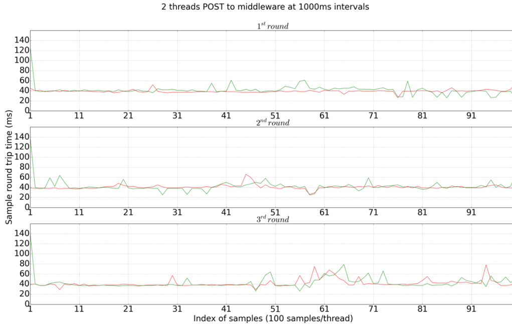
Figure 5-9. Two threads sending 100 POST requests (1000 millisecond delay)
