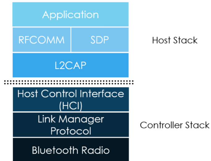
Figure 2-22. a typical Bluetooth stack [13]
