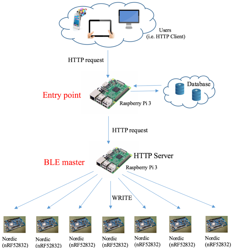
Figure 3-5. Actuating flow
