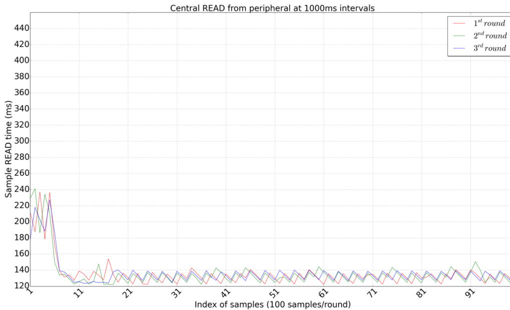
Figure 5-17. 100 sequential reads from an endpoint (1 second delay)
