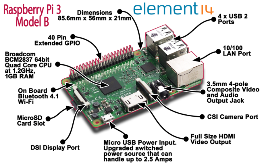
Figure 2-7. Raspberry Pi 3 layout [34]
