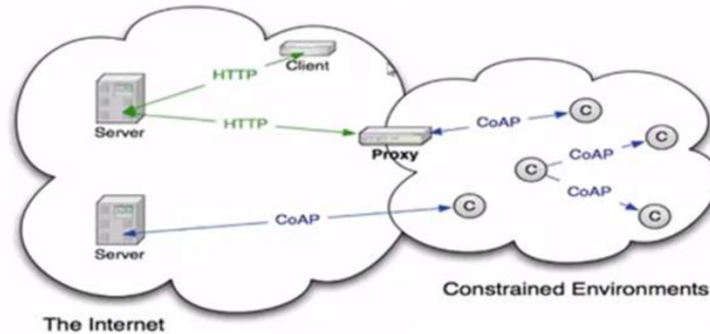
Figure 2-18. CoAP architecture [64]
