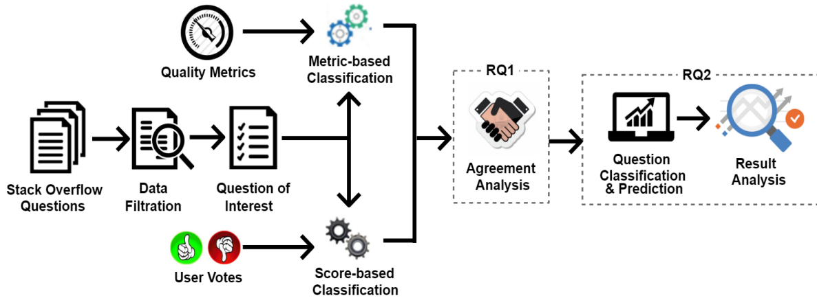
Figure 6.3: Schematic diagram of our study.
