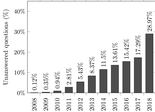
Figure 3.1: Percentage of the questions not answered in SO over eleven years [87].
