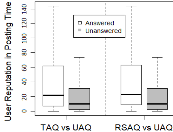
Figure 3.5: User reputation ( TAQ =Total Answered Questions, RSAQ =Randomly Sampled Answered Questions, UAQ =Unanswered Questions).
