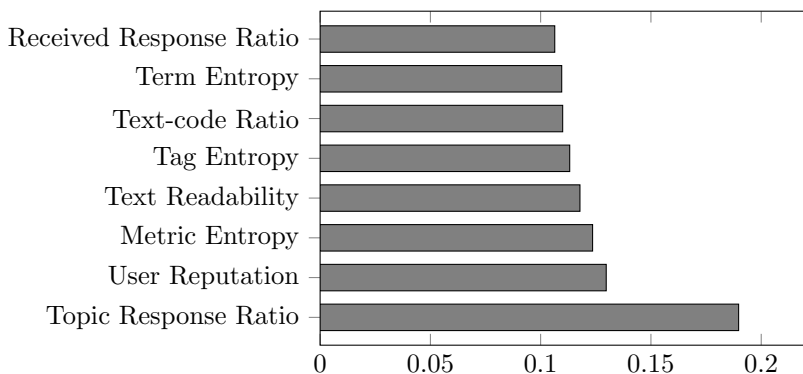
Figure 3.7: Feature Rank
