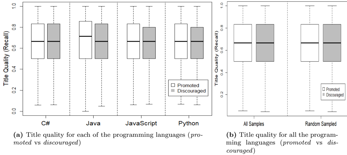
Figure 6.4: Title quality
