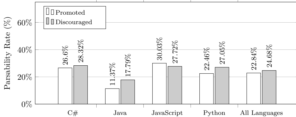
Figure 6.9: Parsability rates of the programming languages (promoted VS discouraged questions).
