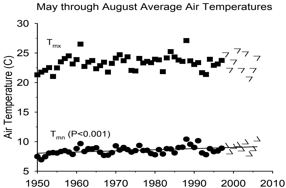
Figure 4: The relationship of the seasonal average maximum (T mx ) and minimum (T mn ) air temperatures for May through August (MJJA) with years. Linear relationship for T mn is between temperature and years from 1950 to 2006. Triangles represent the years from 1998 to 2006.
