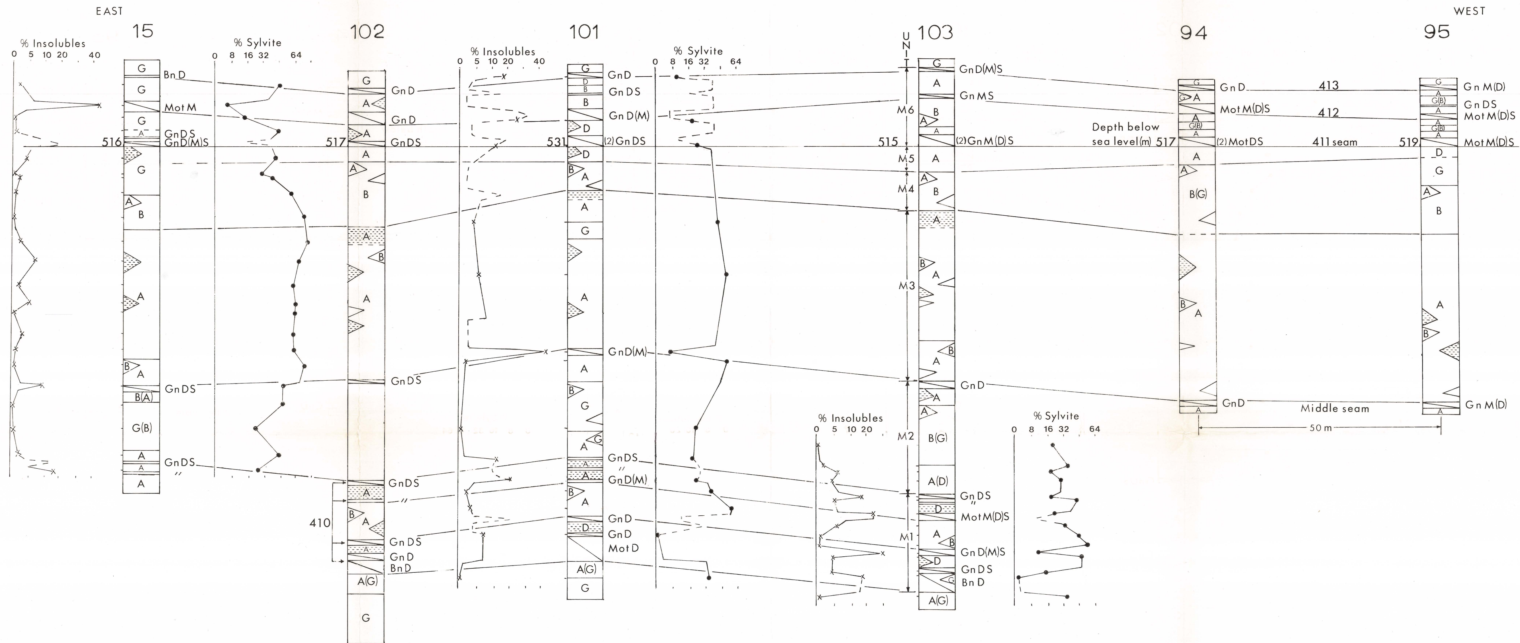
Fig. 4.8 STRATIGRAPHIC CROSS-SECTION OF THE ORE ZONE IN PCS MINING LTD., CORY DIVISION POTASH MINE.
