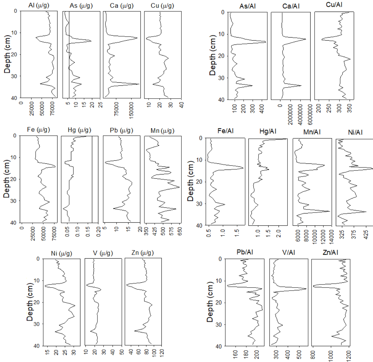
Figure 5.17 Profiles of metal concentrations for Al, Ca, Fe, Mn, As, Cu, Hg, Pb, Ni, V, and Zn in Isadore's Lake, expressed as \mu\text{g/g} (left). Profiles of Ca, Fe, Mn, As, Cu, Hg, Pb, Ni, V, and Zn normalized to Al in Isadore's Lake expressed as the ratio of each metal's concentration to Al concentration (right). A vertical line shows the ISQG concentration for As, 7.24 \mu\text{g/g} .
