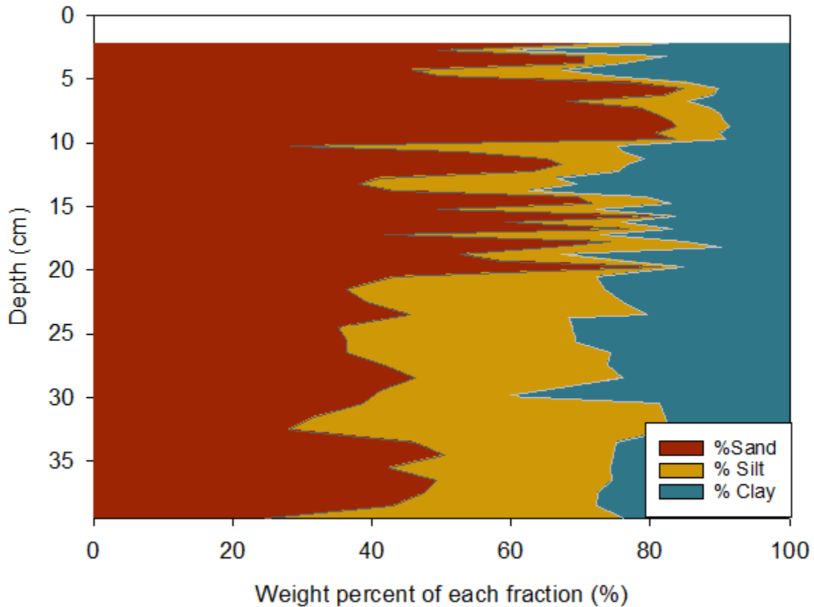
Figure 5.12 Particle size distribution of sediment core II from Isadore's Lake.
