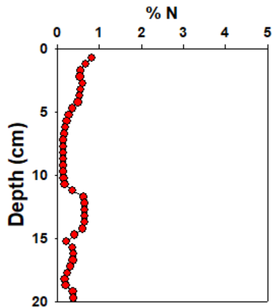
Figure A.4 Total nitrogen content in Isadore's Lake expressed as mass %.
