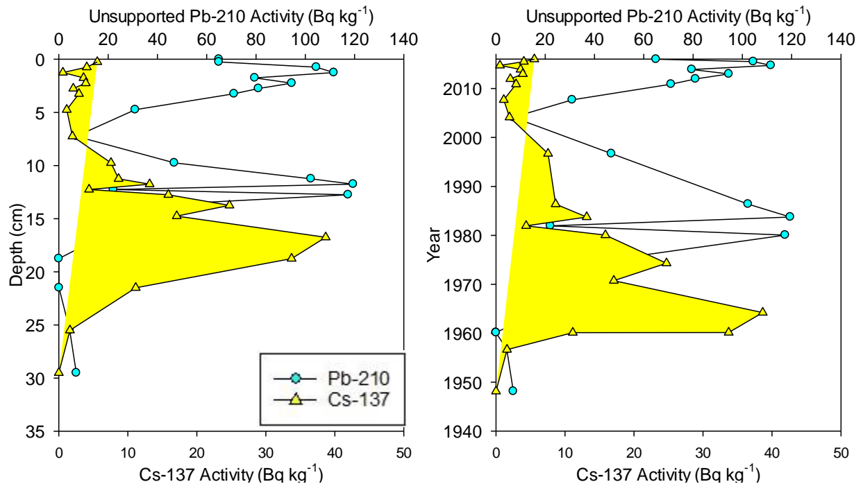
Figure 5.15 Profiles of Pb-210 and Cs-137 for Isadore's Lake (Bq kg -1 ).
