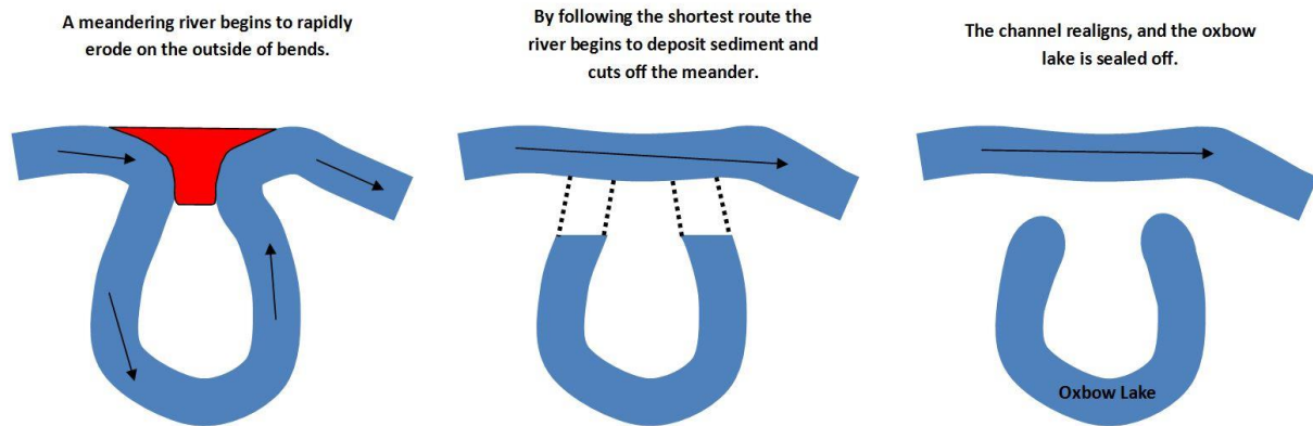
Figure 2.2 Formation of an Oxbow Lake through meander cut-off. Image after (Trenhaile, 1998).
