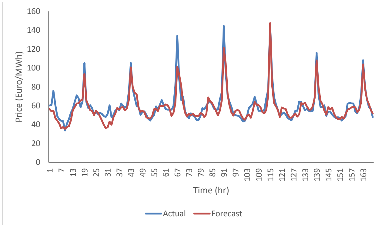
Fig. 3.3 One-week Nord Pool real and simulated day-ahead auction MCP with DSHW model (with spike data points excluded)
