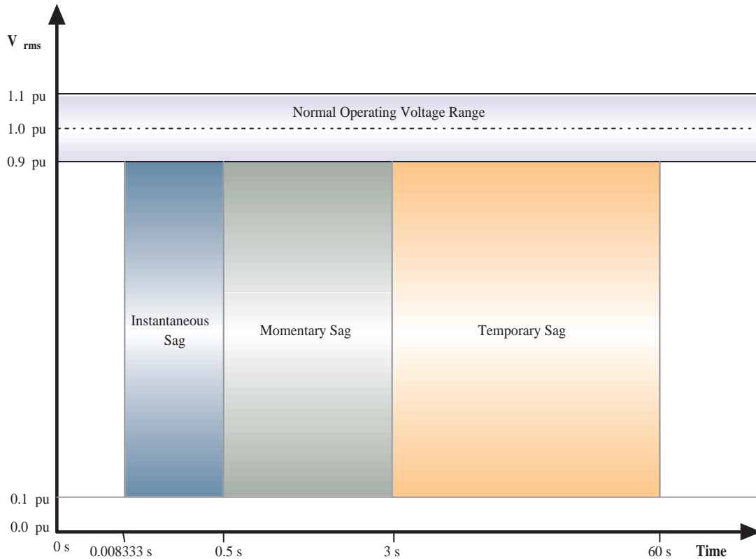
Figure 3.3: Sag Classification
