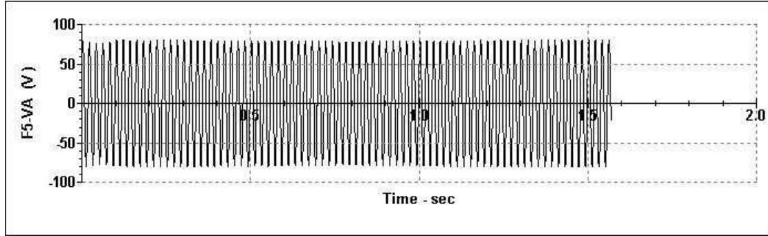
Figure 5.40: Relay Recorded Momentary Sag Waveform
