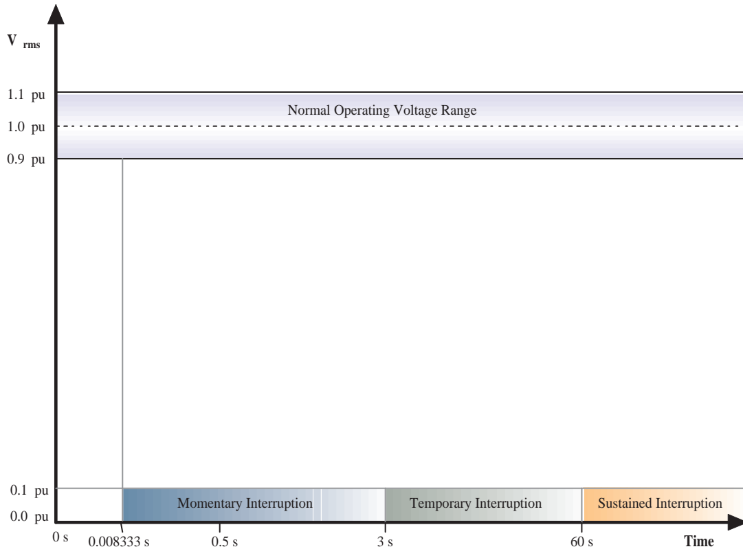
Figure 3.5: Interruption Classification
