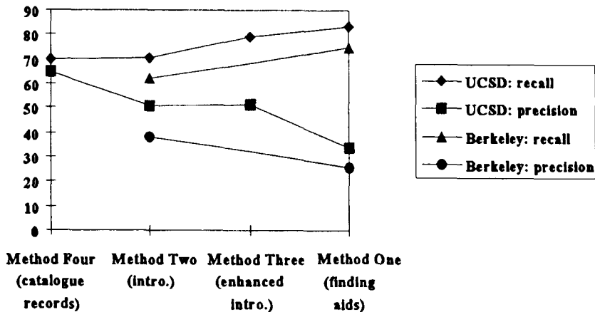
Figure Two Recall and Precision -- Average for Each Method (%)
